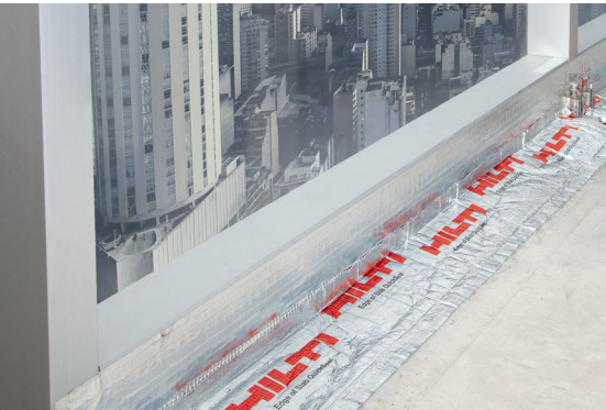
Fig. 34: Comparison between CFS-EOS QuickSeal vs traditional method
