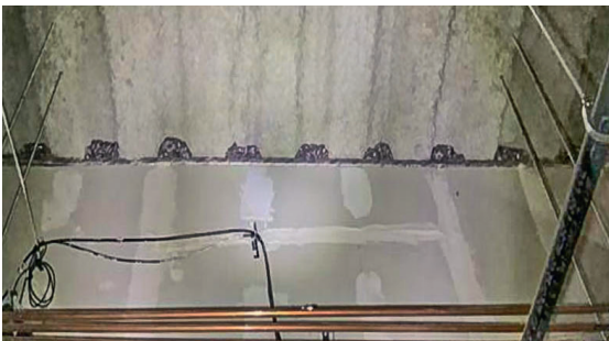
Fig. 26: Hilti CFS-TTS MD installed correctly per EJ
