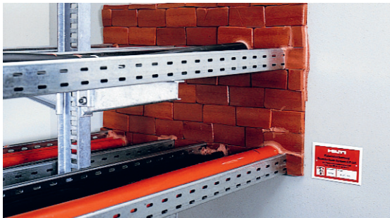
Fig. 8: Preformed firestop block, Hilti CFS-BL Firestop Block used for sealing large openings with multiple through penetrations. The firestop block should be stacked with staggered seams within the opening
