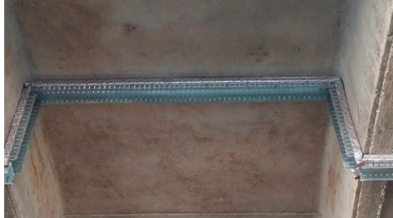
Fig. 25: Hilti CFS-TTS used on top of wall joint
