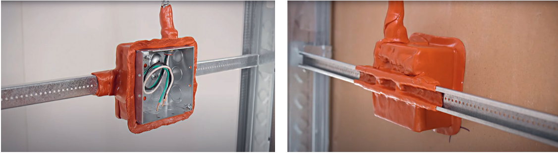
Fig. 21: Putty pad, Hilti CP 617, for sealing electrical box inside walls.
