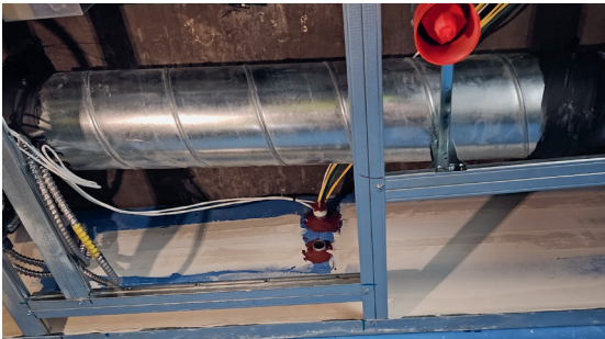
Fig. 16: Blank opening (bottom one out of two sealed small openings)
