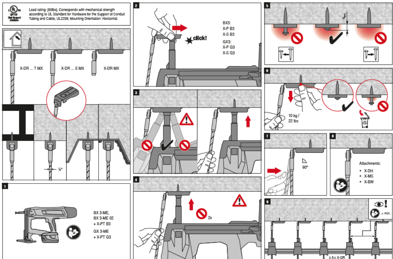
FIGURE 7 – X-DR MX INSTALLATION INSTRUCTIONS
